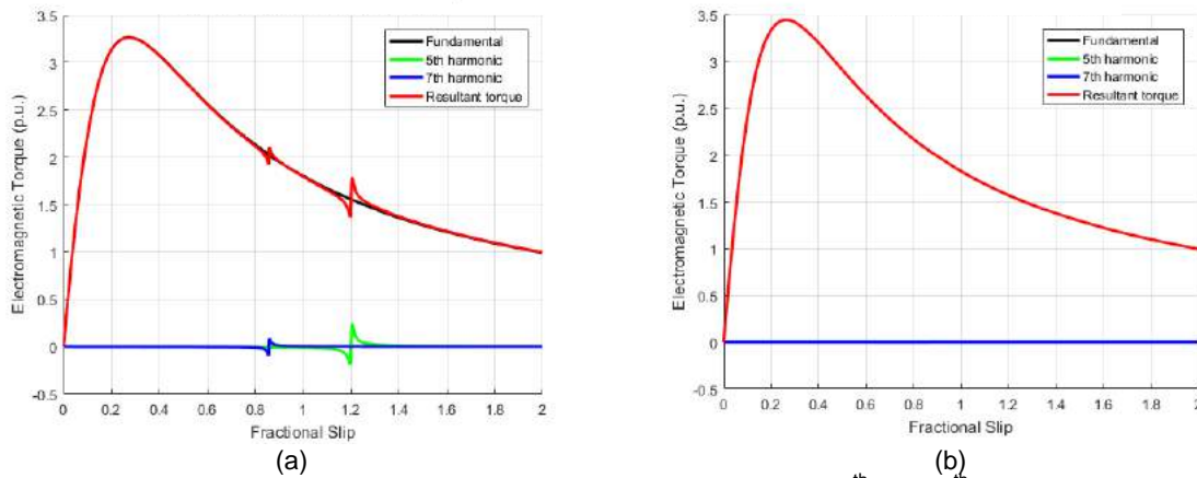
Fig. 31. Approximate motor electromagnetic torque curve considering the 5 th - and 7 th -order space harmonics of MMF: (a) original single-layer winding (Case 0); (b) optimized double-layer winding (Case 3).
