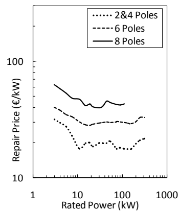
Fig. 7. SCIM repair prices per kW in a typical European repair shop including stator rewinding, standard bearing replacement, rotor dynamic calibration, painting and basic quality control tests.
