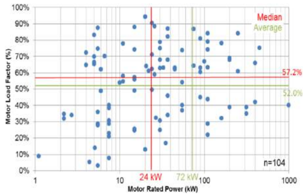
Fig. 5. Data on SCIM load factor in the industrial sector, 2013 (104 data points) [9].
