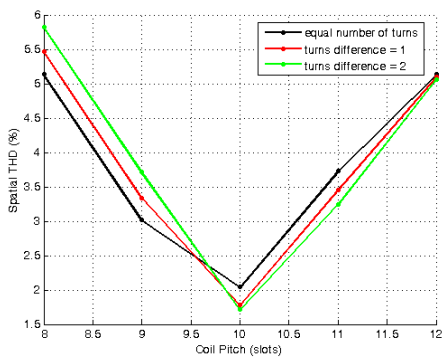
Fig. 25. MMF spatial THD as a function of the coil pitch for a 48-slot, 48-turn/coil, eccentric, double-layer winding.
