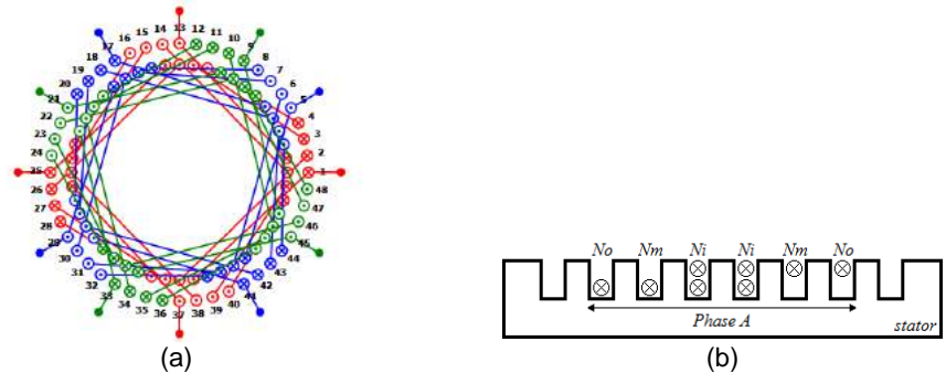
Fig. 24. Concentric, double-layer, 3-tier, stator winding configuration: (a) circular scheme; (b) identification of inner and outer coils.
