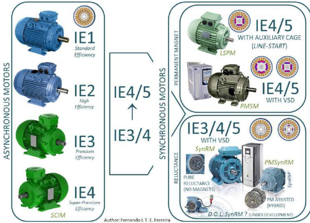
Fig. 2. Overview of the three-phase motor technologies available in the market and/or under development [6].
