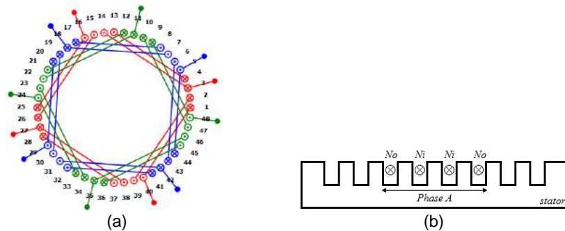
Fig. 22. Concentric, single-layer, 3-tier, stator winding configuration (original): (a) circular scheme; (b) identification of inner and outer coils.
