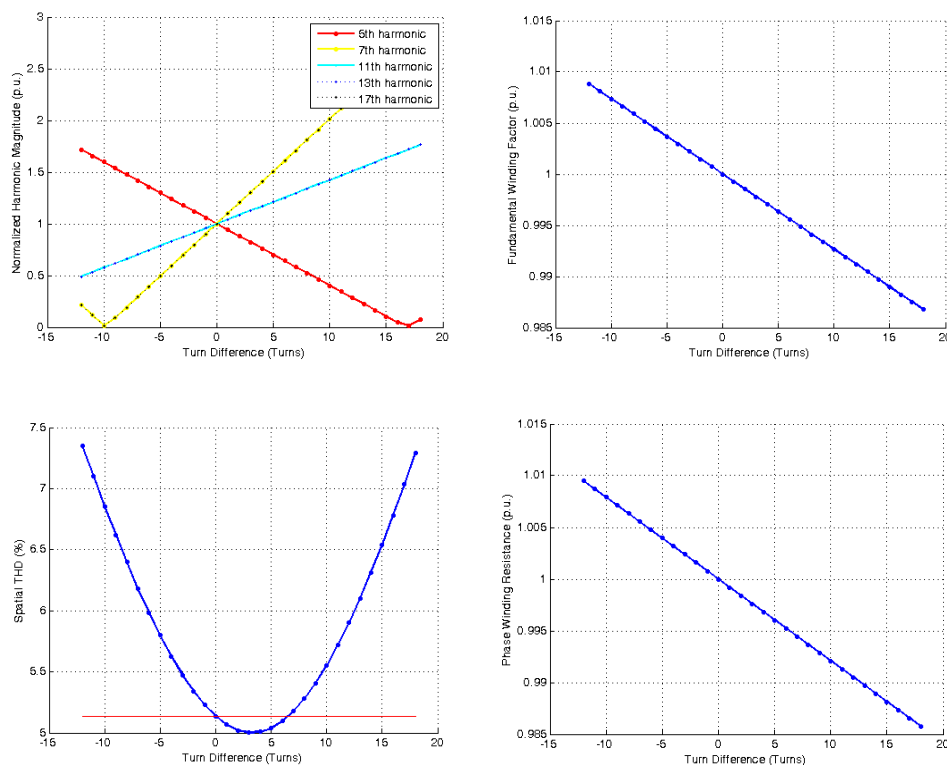
Fig. 23. MMF space harmonics (normalized in relation to the fundamental) and THD as a function of the turn difference, for a 48-slot, 48-turn/coil, concentric, single-layer winding.
