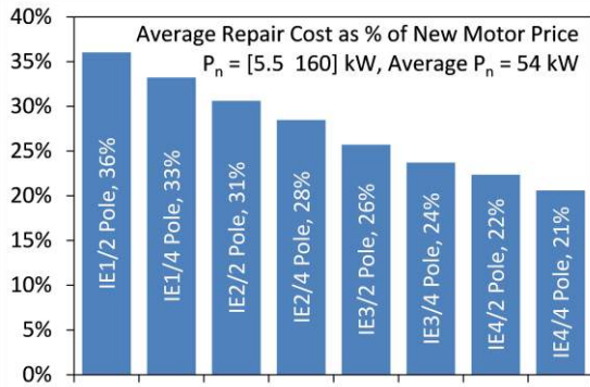
Fig. 8. Average repair cost as a percentage of new motor price.
