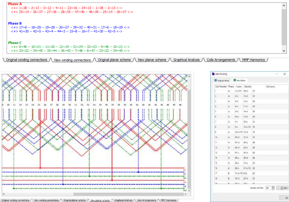
Fig. 17. Numerical and planar representation of the windings and coils.
