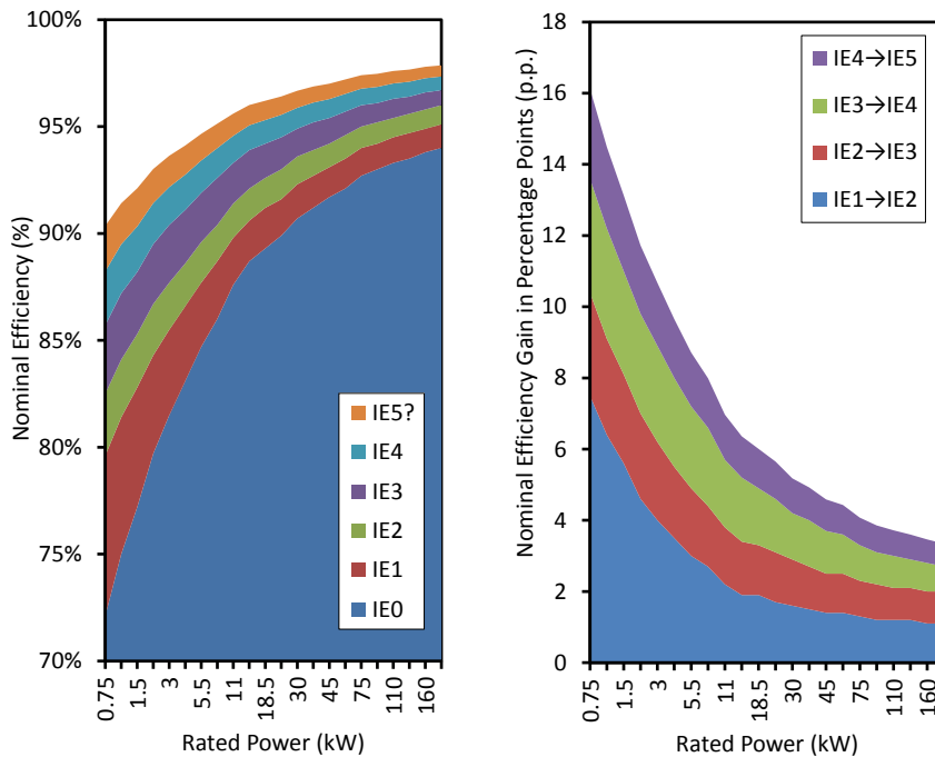
Fig. 3. Motor efficiency classes defined by IEC60034-30-1 standard for 4-pole, 50-Hz, single-speed motors in the 0.75-200 kW power range: (left) nominal efficiency limits; (right) nominal efficiency gain [2, 7, 8].
